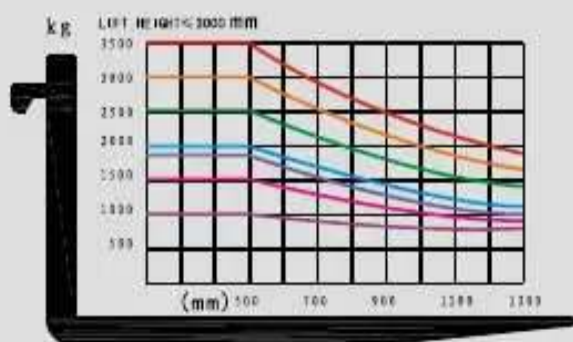
Load Chart
